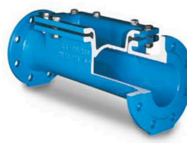
Hatch box with flanged connection for cleaning and inspection
