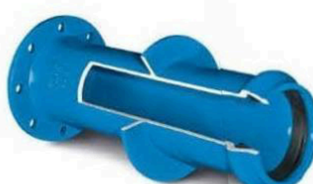
E-KS 600 expansion joint 600 mm long with puddle flange
